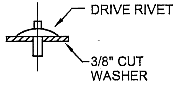
DRIVE RIVET DETAIL FOR MOUNTING SIGN
