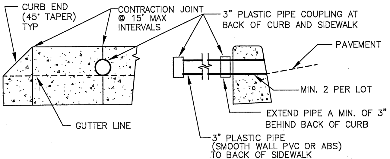
WEEP HOLE THROUGH CURB
